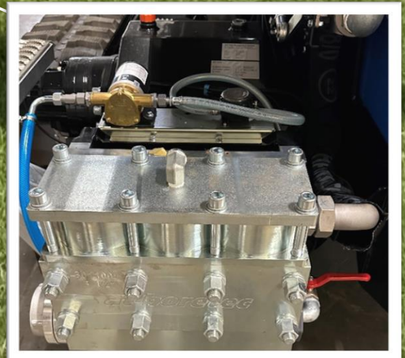
Low Flow mud pump with 660 ltr. / min. @ 270 rpm
